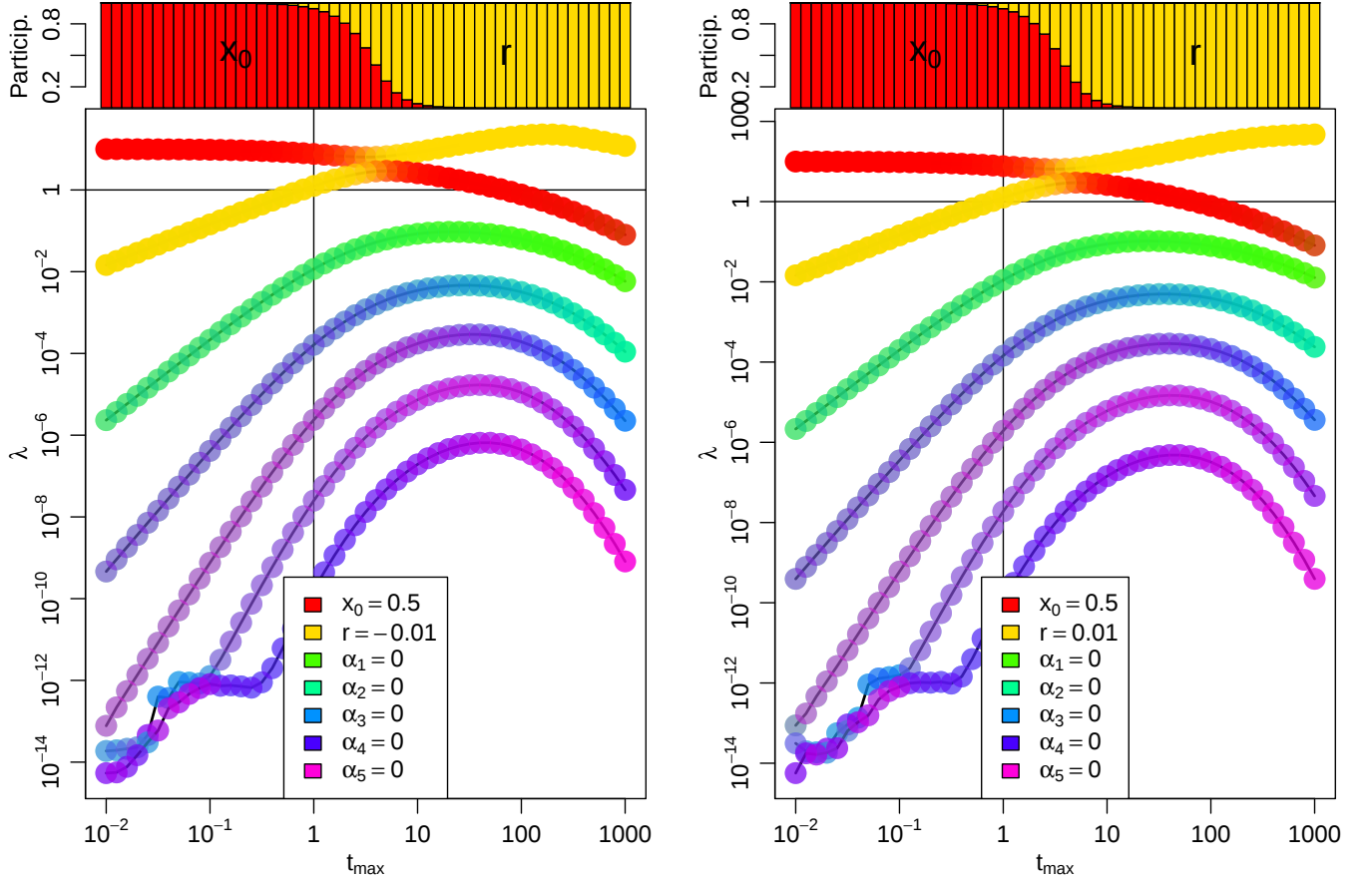
FIG. 5. TWIG analysis near-but-not-at the bifurcation values show the diagnostic pattern of an increasing eigenvalue at intermediate time scales, but then a decrease (in A) or an asymptote (in B; top yellow curve in the t_{max}=100 to 1000 range in both). It is still relatively easy to identify bifurcation parameters and the bifurcation's codimension, though the fall-off becomes more pronounced, and thus the clarity of the analysis more obscured, the further one moves away from the bifurcation in either direction.
