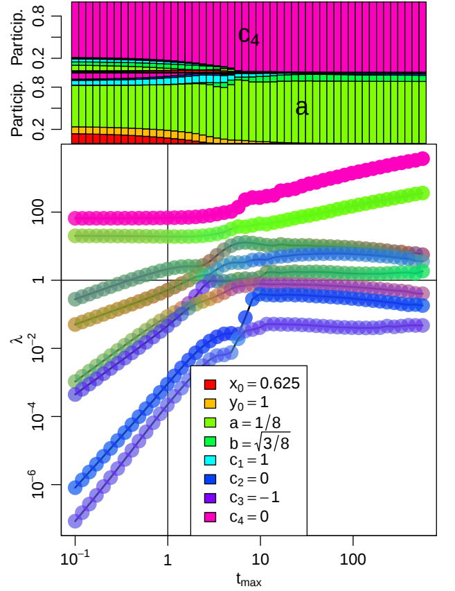
FIG. 9. Analysis of the “glycocoillator” bifurcation (Eq. 11). The frequency of the oscillations are driven by c_4 , while the radius of oscillations can be controlled with just one of the a, b parameters discovered by Sel’kov [43].
