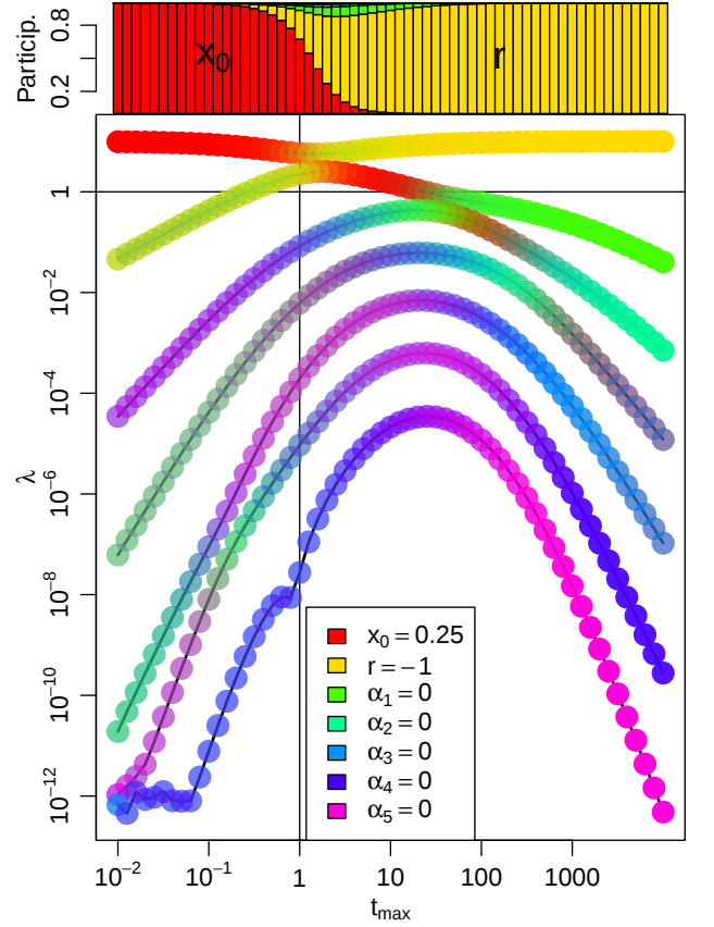
FIG. 7. Equations such as Eq. (9) that are not in normal form can be interpreted using the same procedure as for normal form bifurcations. As above, the presence of just one non-decreasing eigenvalue, whose corresponding eigenvector is dominated by the single parameter r , indicates that the system has codimension 1 and the bifurcation parameter involves only r . The relevant (not hyperrelevant) leading eigenvalue is characteristic of a transcritical bifurcation.
